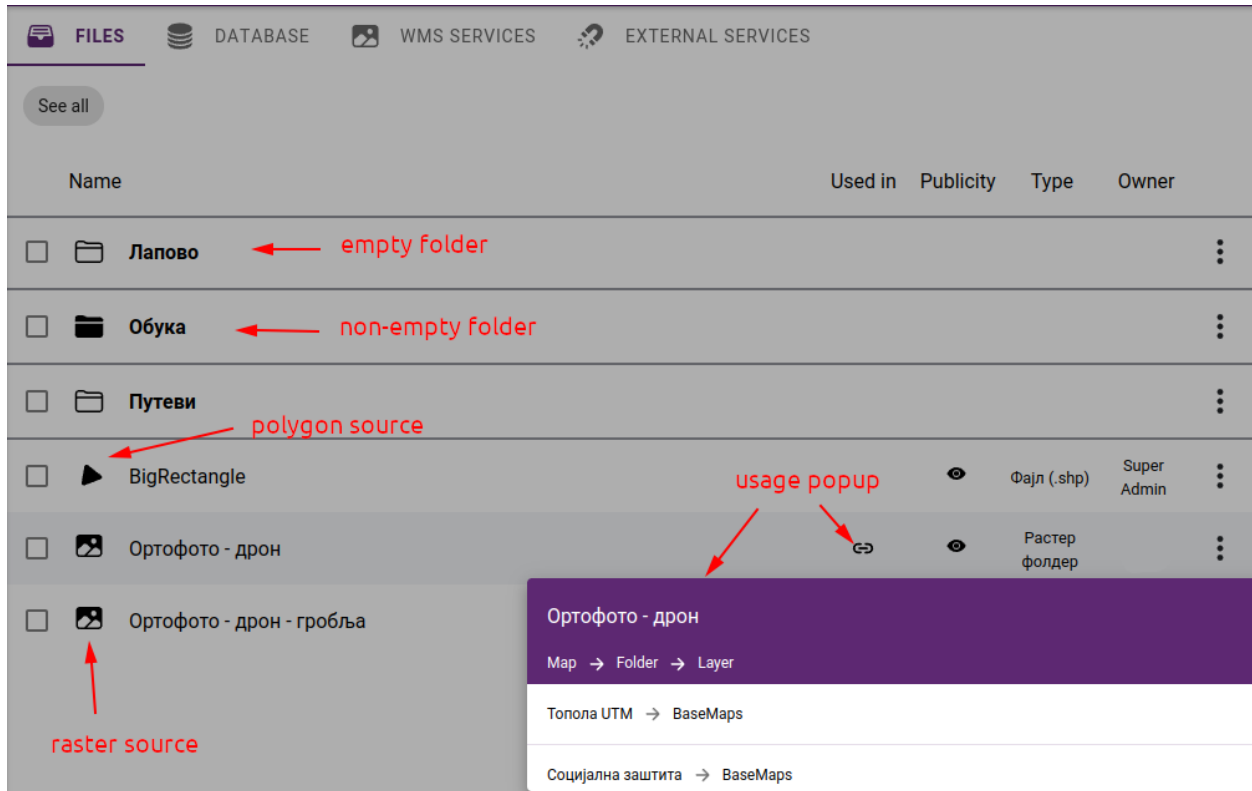
Slika 35: Data source folder contents by opening the usage pop-up window
