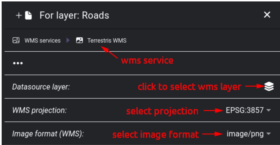
Slika 68: WMS service selected
